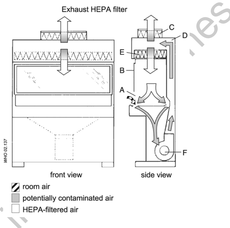
Fig. 4. Schematic representation of a Class IIA1 biological safety cabinet. A: front opening, B: sash, C: exhaust HEPA filter, D: rear plenum, E: supply HEPA filter, F: blower.
